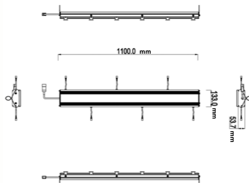
Structure chart of Driver Box
