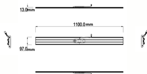
Structure chart of Bar Light
