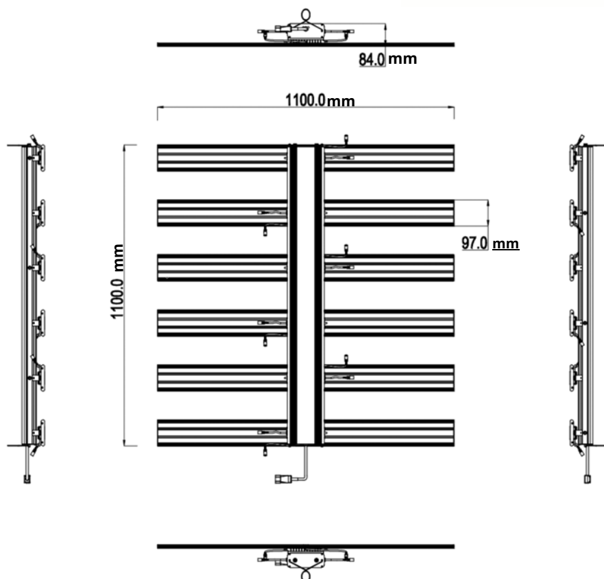
Structure chart of Light Fixture
